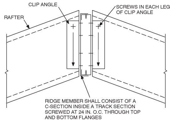
FIGURE R804.3.3.1 RIDGE BOARD CONNECTION
