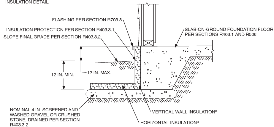
INSULATION DETAIL
