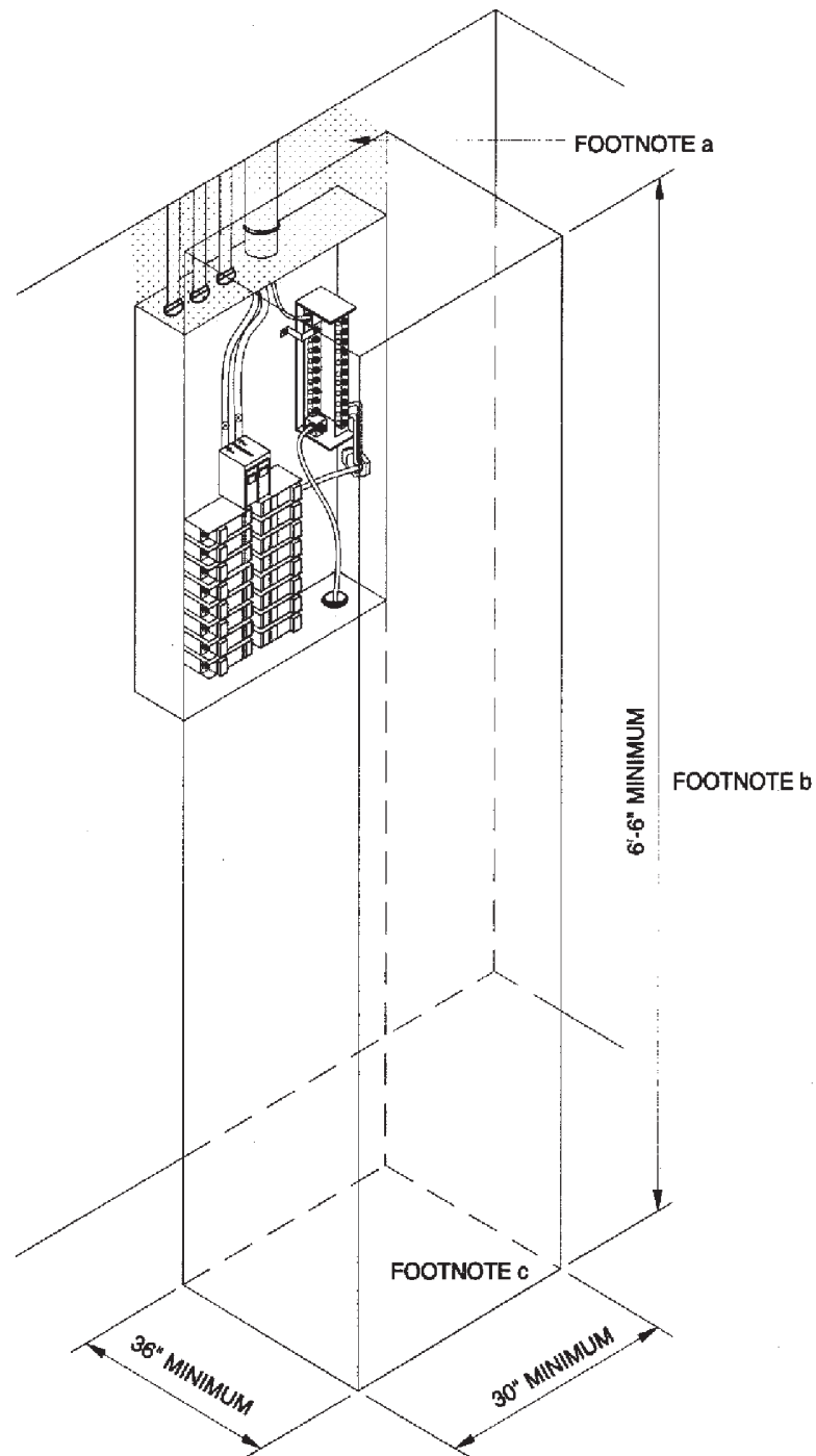
FIGURE E3305.1 a,b,c,d,e WORKING SPACE AND CLEARANCES
