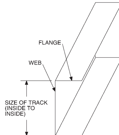
FIGURE R505.2(2) TRACK SECTION
