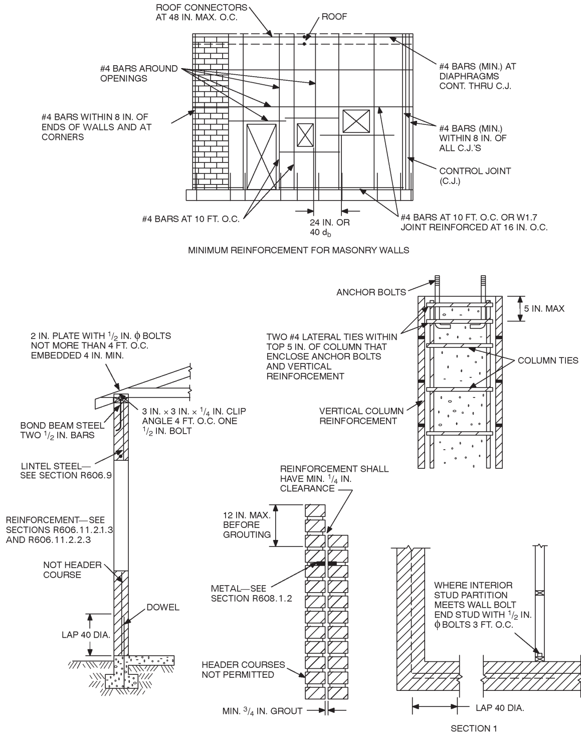
FIGURE R606.10(2) REQUIREMENTS FOR REINFORCED GROUTED MASONRY CONSTRUCTION IN SEISMIC DESIGN CATEGORY C
