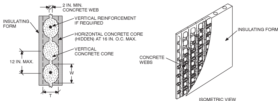
FIGURE R611.4 WAFFLE-GRID ICF WALL SYSTEM
