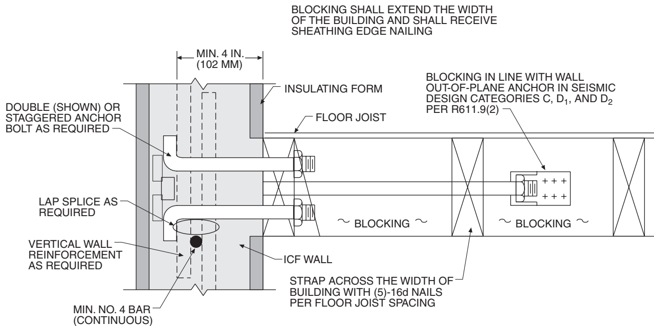
FIGURE R611.8(7)
